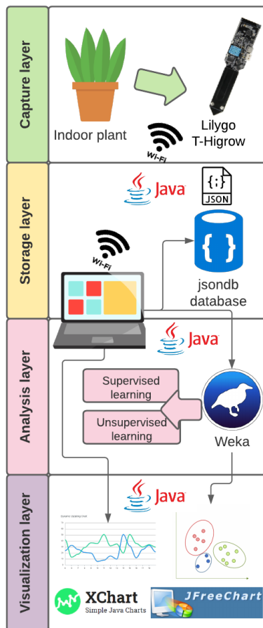
Fig. 5. Implementation view
