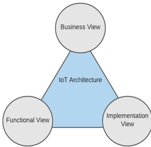
Fig. 2. Architecture views
