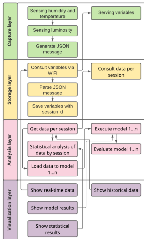
Fig. 4. Functional view
