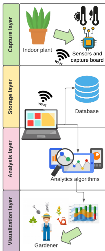
Fig. 3. Business view
