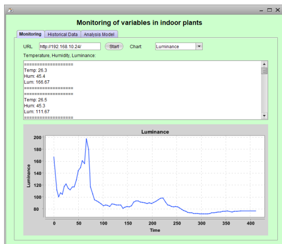
Fig. 6. Monitoring tab
